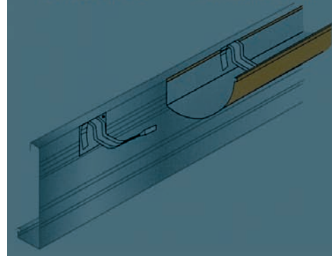
LEFT HAND STOP END
